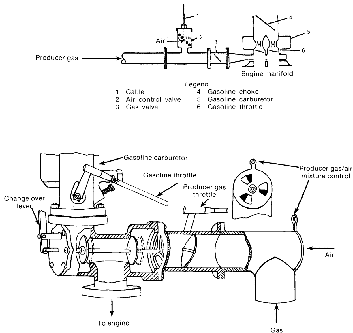
Fig. 11-3. Gas air mixers (Source: Adapted from Cash 1942 and Anon 1943)
