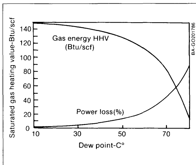
Fig. 8-21. Power loss due to moisture saturated producer gas for 150 Btu/scf dry basis gas
