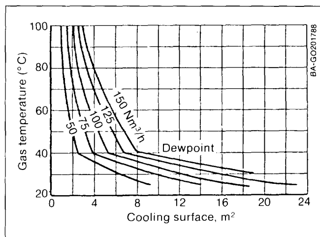
Fig. 8-23. Gas cooler surface requirements for various outputs at 700°C (Source: Gengas 1950, Fig. 99)
