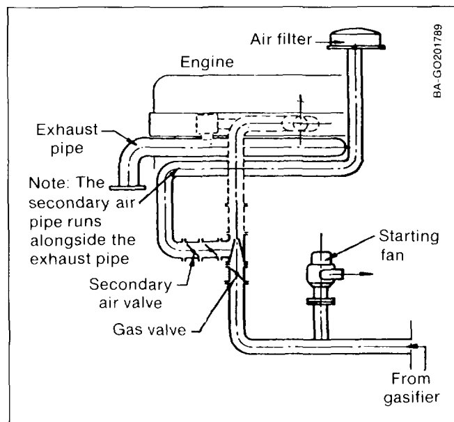
Fig. 8-25. Heating of secondary air by exhaust gas heat from the engine (Source: Gengas 1950, Fig. 85)
