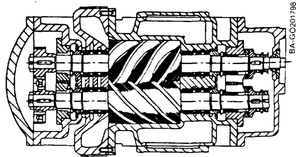
Screw-type rotary compressor.
