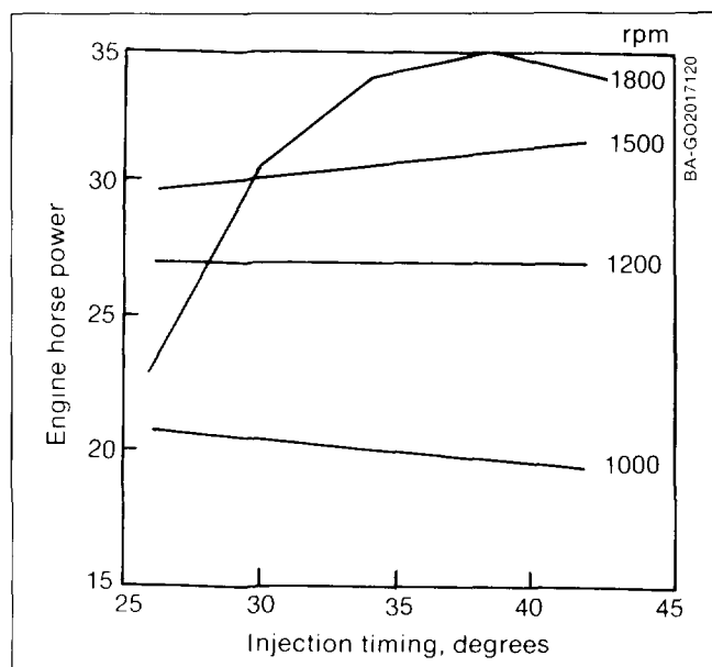
Fig. 11-12. Optimum injection timing for pilot diesel dual fuel (Source: Kaupp 1984a, Fig. 210)
