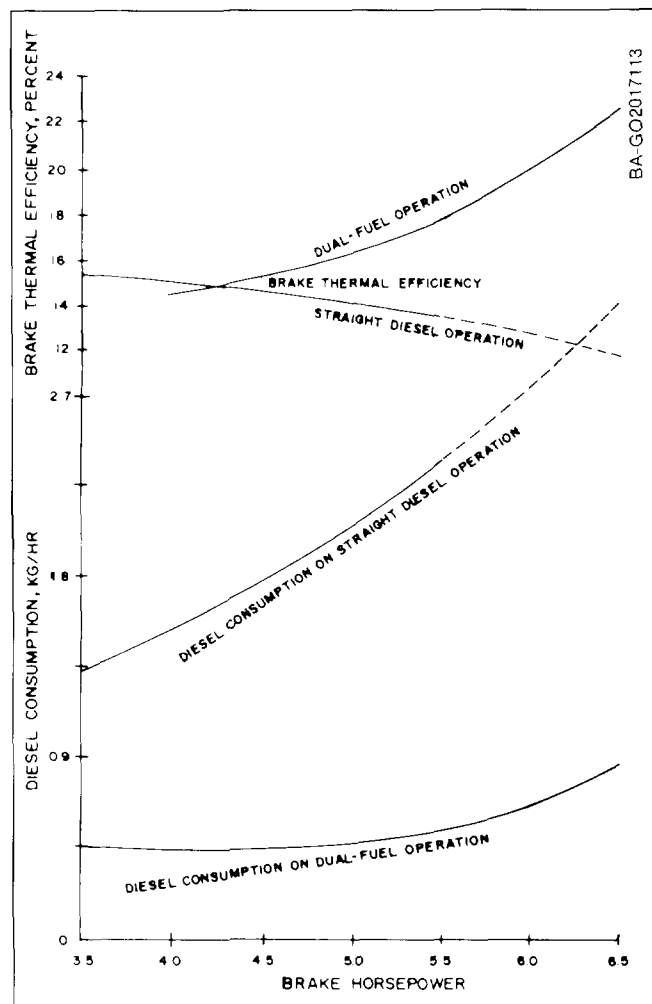
Fig. 11-11. Diesel dual-fuel efficiency and fuel savings (Source: Cruz 1983, Fig. 14. © 1973. Used with permission of the Beijer Institute)
