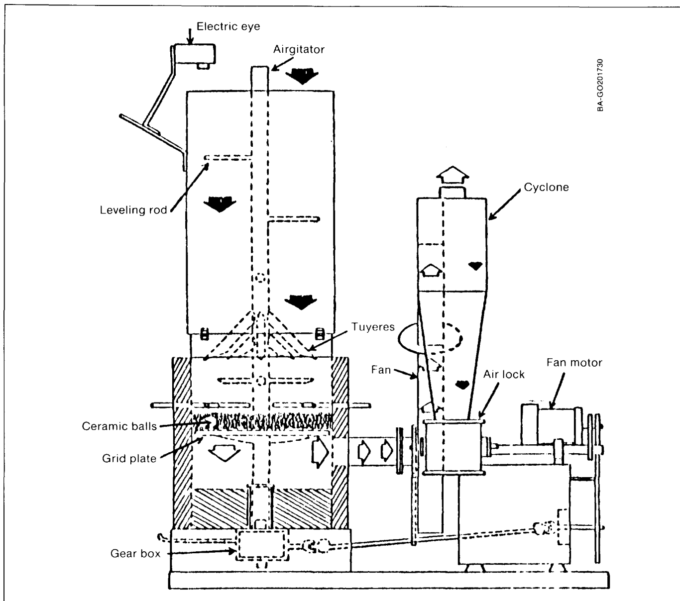
Fig. 5-11. Buck Rogers gasifier (Source: Walawender 1985, p. 913. © 1985. Used with permission of Elsevier Science Publishing Co., Inc.)
