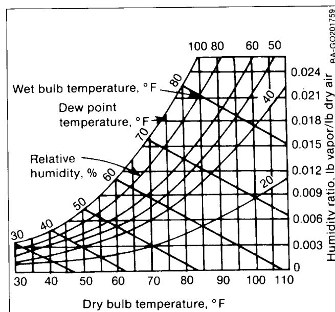
Fig. 7-18. Psychrometric chart for medium temperatures (Source: Adapted from ASHRAE 1981)
