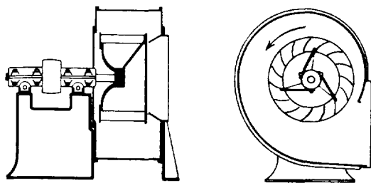
Backward-curved-blade fan.
