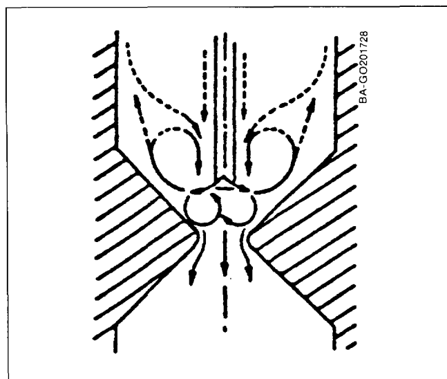
Fig. 5-9. Downdraft center nozzle gas producer (Source: Groeneveld 1980a)
