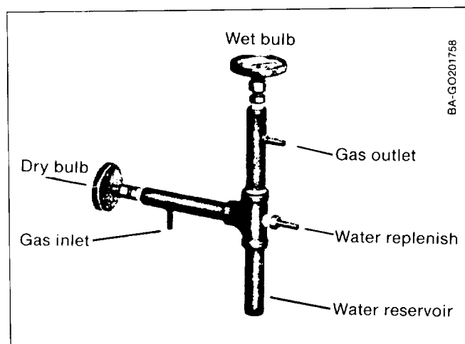
Fig. 7-17. Gas stream hygrometer (Source: RAC, p. 7)
