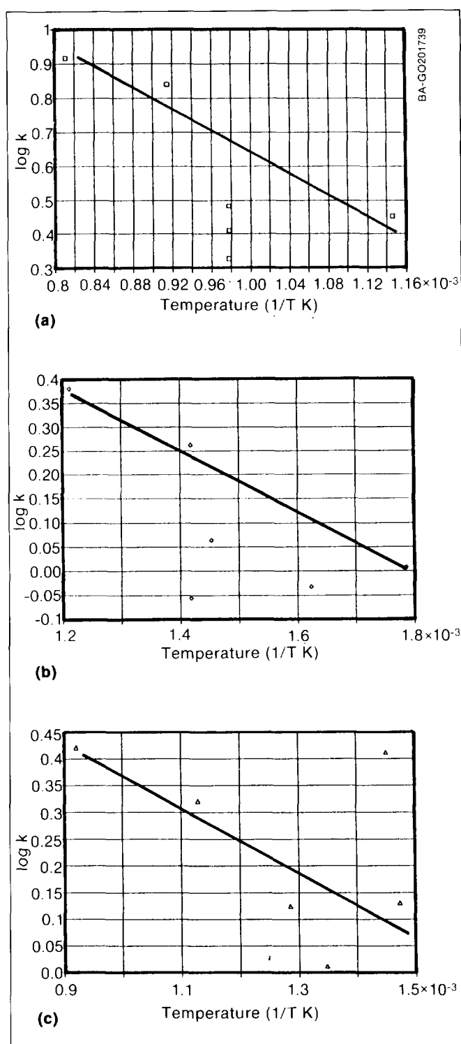
Fig. 5-20. Kinetic rate of tar cracking for (a) dolomite lime, (b) Si-Al cracking catalyst, and (c) silicalite cracking catalyst
