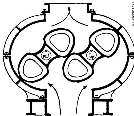
Two-impeller type of positive rotary blower.
