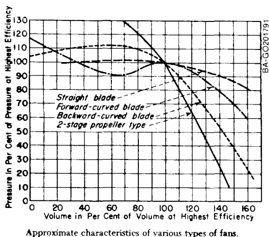
Fig. 9-5. Centrifugal blowers (Source: Perry 1973, Figs. 6-37, 6-38, 6-39, 6-41. © 1973. Used with permission of McGraw Hill Book Co.)
