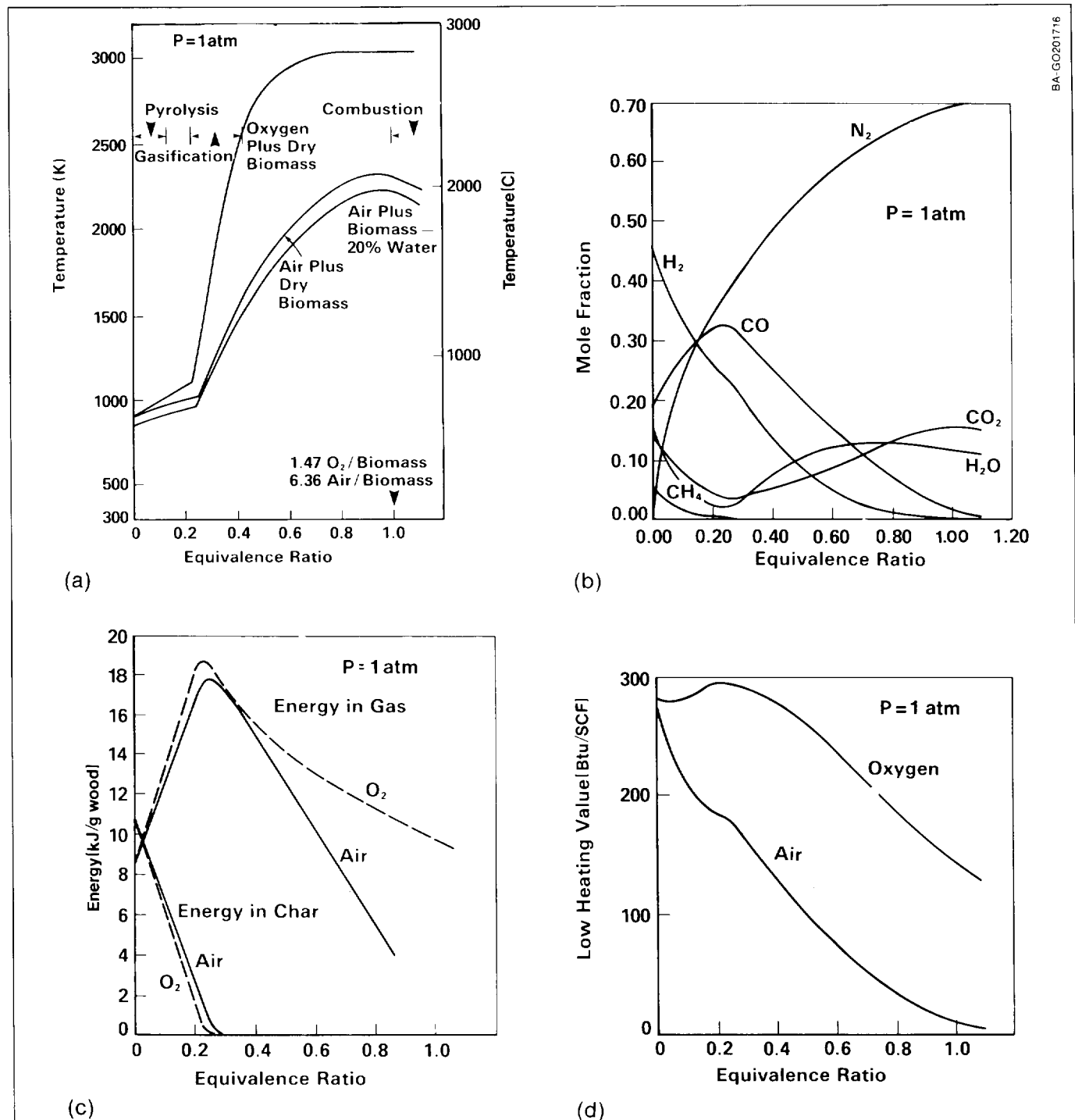
Fig. 4-4. (a) Adiabatic reaction temperature for biomass of atomic composition \text{CH}_{1.4}\text{O}_{0.6} reacting with oxygen and air, plotted against the equivalence ratio, \phi , the ratio of oxygen to that required for complete combustion (b) Equilibrium gas composition for reaction with air (c) Energy in solid and gas (d) Energy per volume of gas (Source: Reed 1981, Figs. S-2 - S-5)
